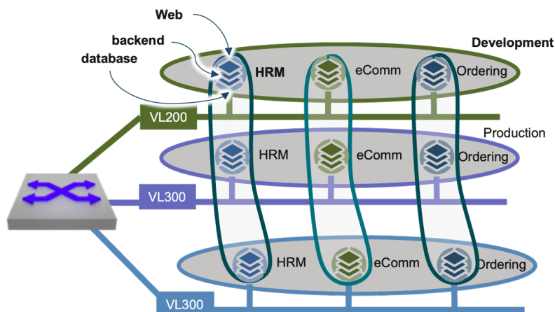
Figure 22: Sample Data Center Topology with MSS Groups of Application Workloads
