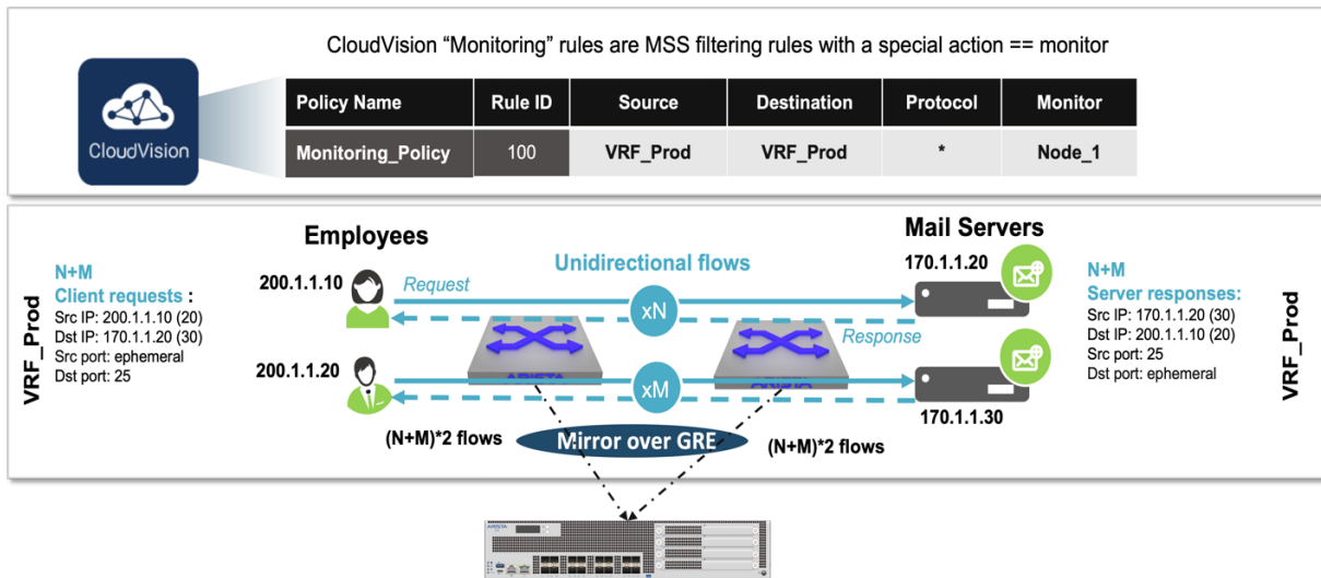
Figure 12: Stateful Observability
