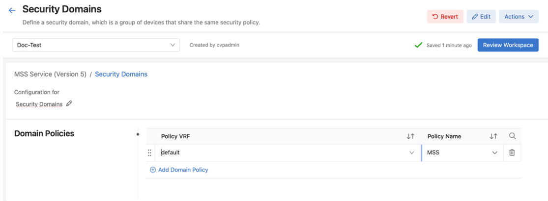
Figure 16: Security Domains
