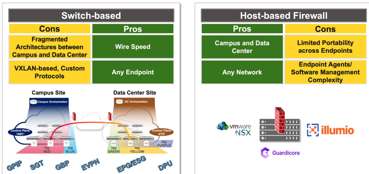
Figure 1: Switch-based vs. Host-based Solutions
