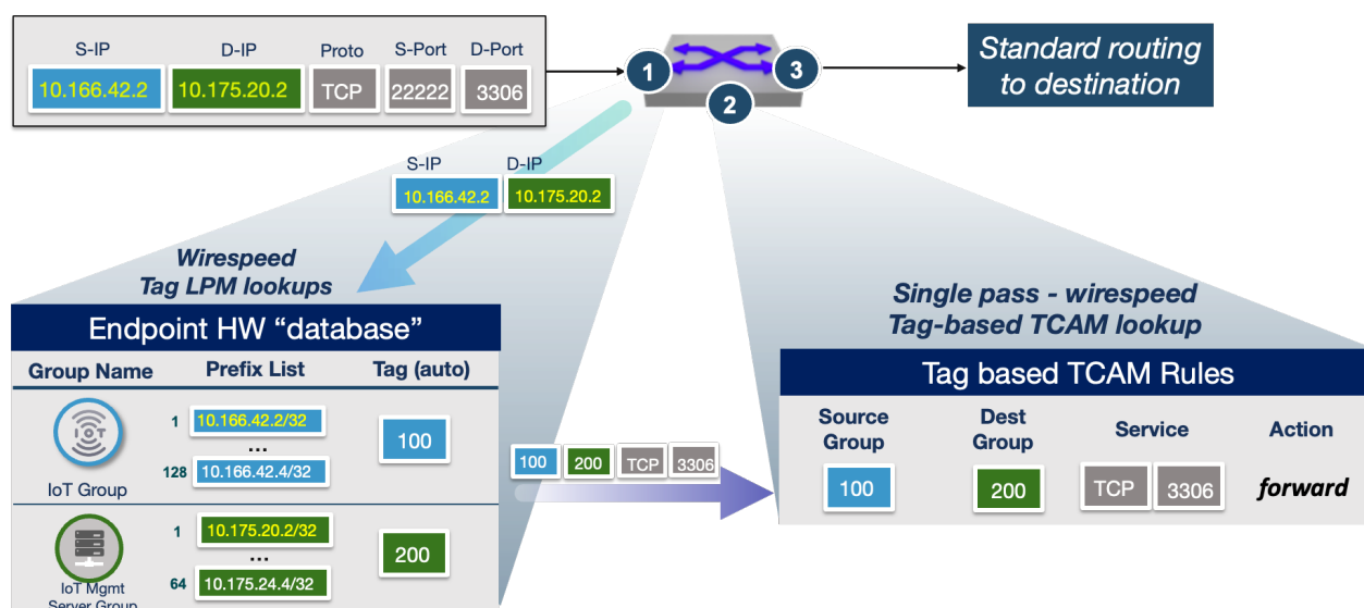
Figure 24: Dynamic Action Enforcement of the Arista MSS Group Tagging Technology
