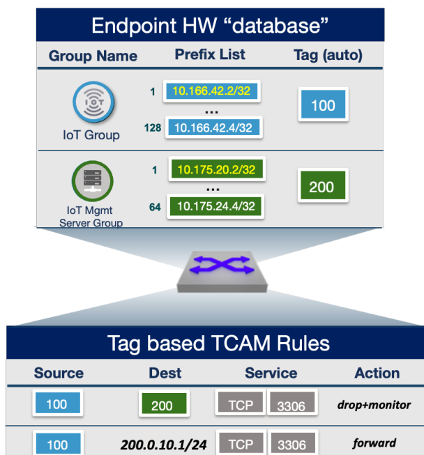
Figure 23: Internal Tag/Label Use in Hardware-based Policy Rules
