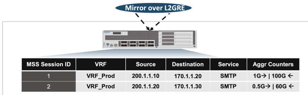
Figure 13: Session Summarization
