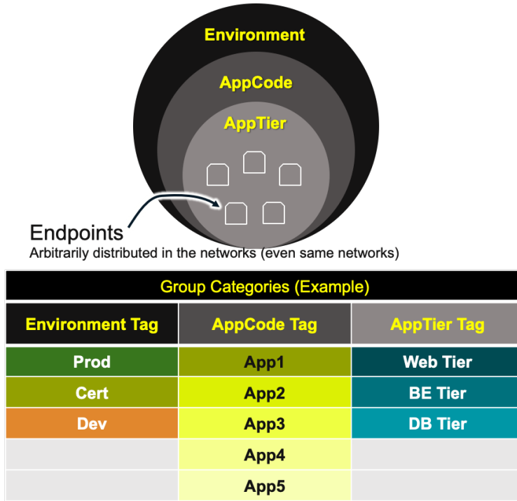
Figure 25: Multi-label Mapping
