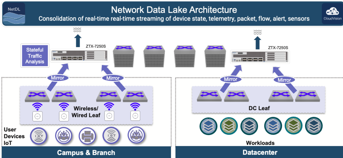
Figure 11: ZTX-7250S Logical Deployment Model
