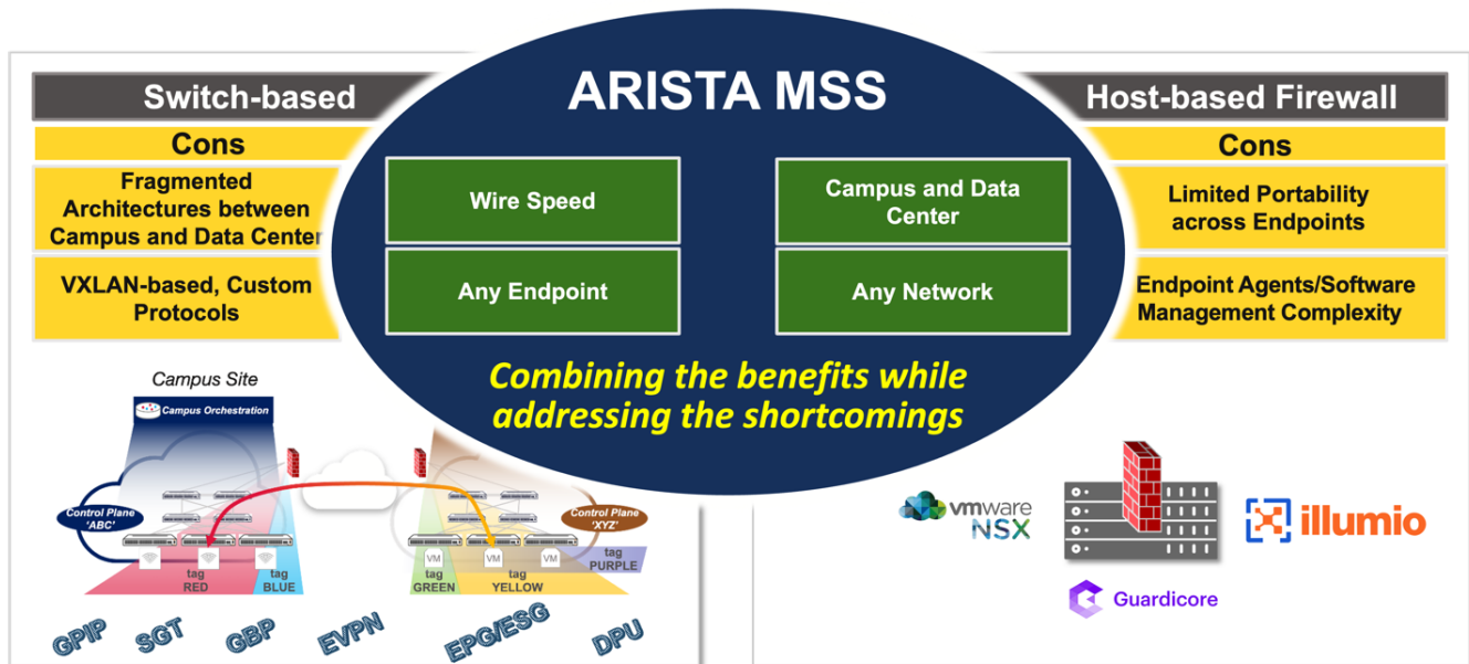
Figure 3: Advantages of Arista MSS's Unified Segmentation Architecture
