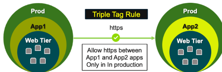
Figure 29: Triple-tag Rule with Three Levels of Filtering
