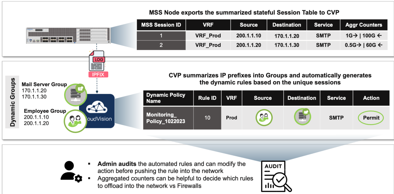
Figure 14: Policy Orchestration and Audit
