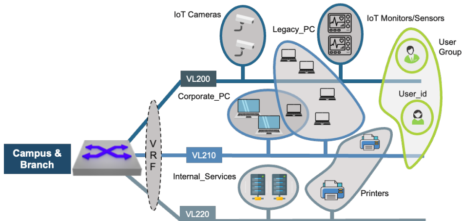
Figure 21: Sample Campus Branch Topology with MSS Groups of Users, Office and IoT Devices
