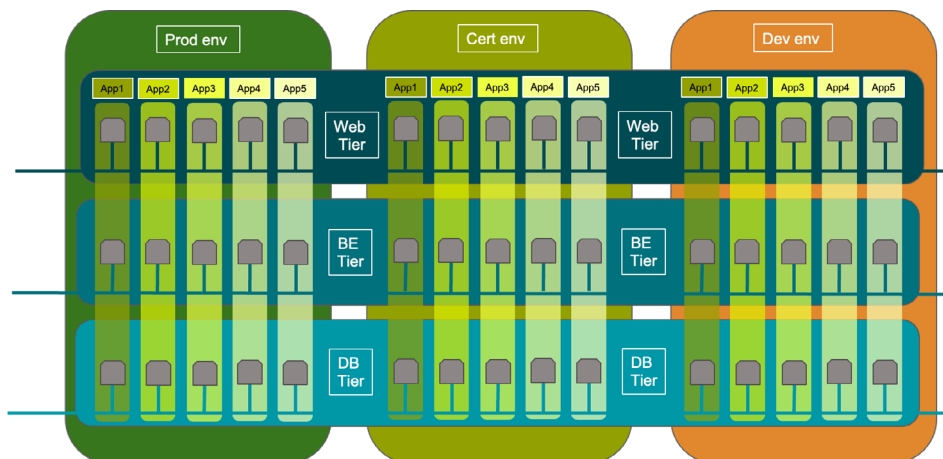
Figure 26: Sample Network Divided into Three Environments
