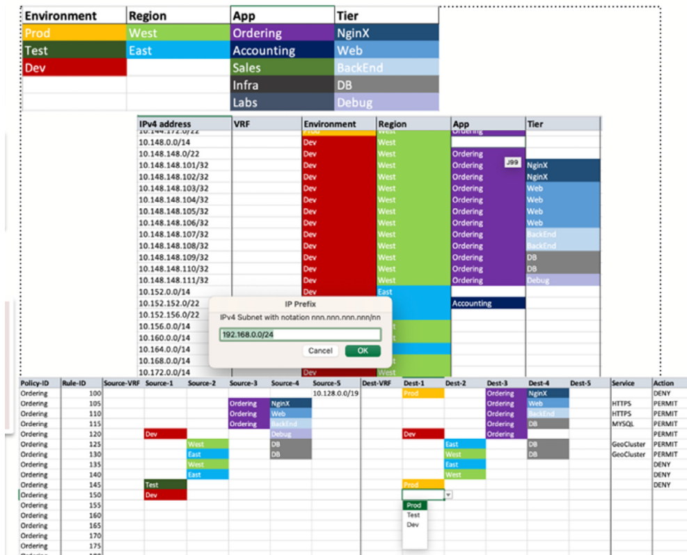
Figure 9: MSS Planner Tool
