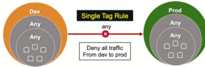
Figure 27: Rule Blocking Communication between Dev and Prod
