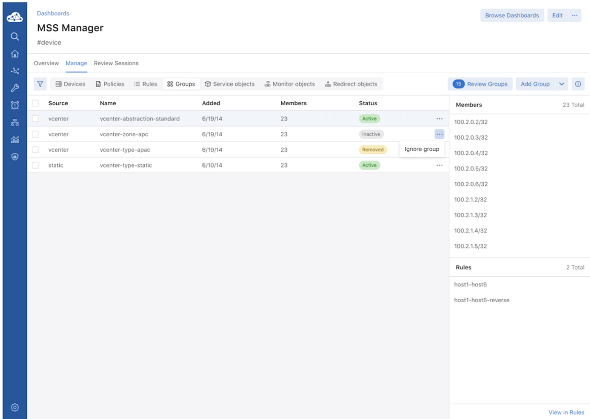
Figure 15: Groups in MSS Manager Dashboard
