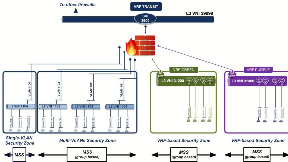
Figure 4 : MSS Technology Deployment
