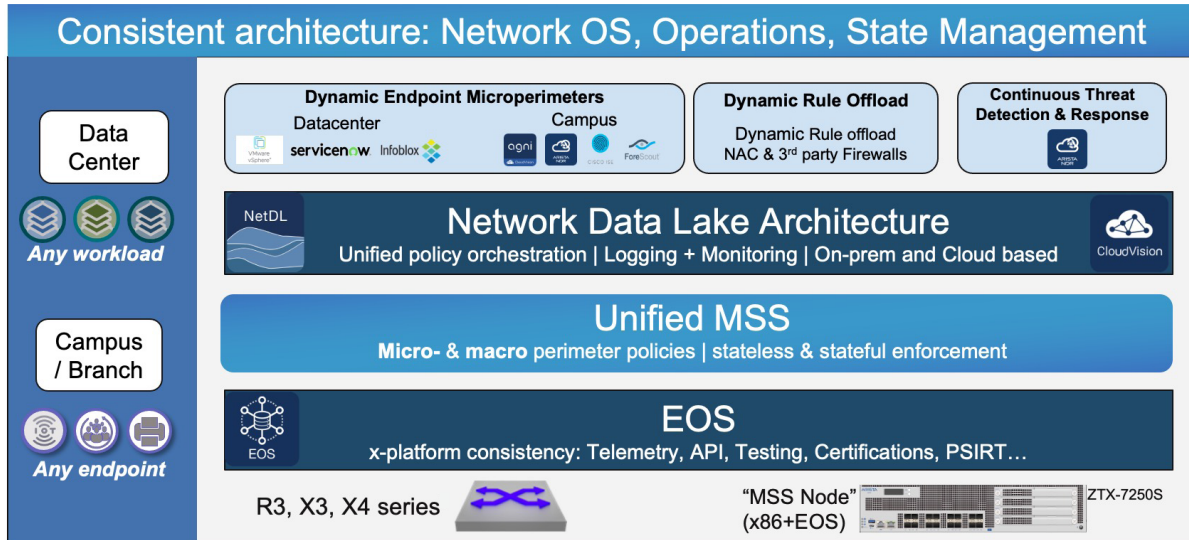
Figure 2: Arista Multi-domain Segmentation Architecture
