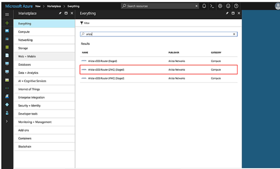
Figure 2: Arista selection
